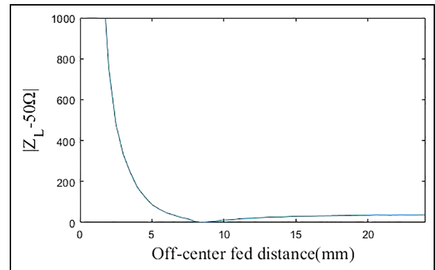
Figure 8. The |Z_L - 50 \Omega| value under different off-center fed distance.
