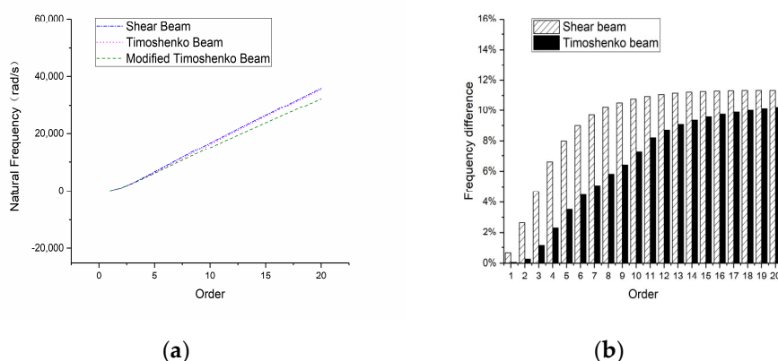
Figure 20. Natural frequencies of the 4-m-long beam: (a) overall frequency curve and (b) frequency difference compared with a modified Timoshenko beam.
