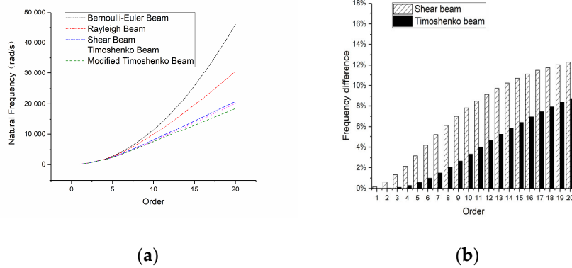
Figure 4. Natural frequencies of the 8-m-long beam: (a) overall frequency curve and (b) frequency difference compared with a modified Timoshenko beam.
