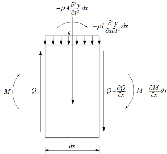
Figure 2. Free body diagram for a differential element.
