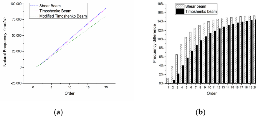
Figure 24. Natural frequencies of the 2-m-long beam: (a) overall frequency curve and (b) frequency difference compared with a modified Timoshenko beam.
