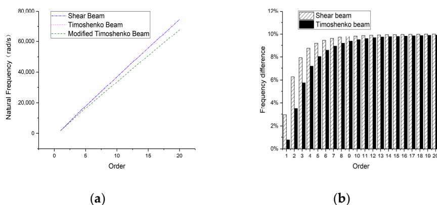
Figure 15. Natural frequencies of the 2-m-long beam: (a) overall frequency curve and (b) frequency difference compared with a modified Timoshenko beam.
