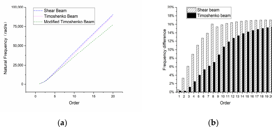
Figure 30. Natural frequencies of the 2-m-long beam: (a) overall frequency curve and (b) frequency difference compared with a modified Timoshenko beam.
