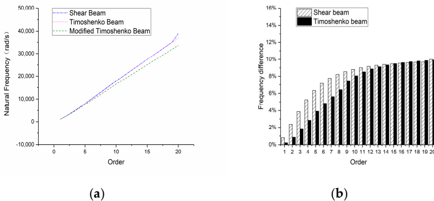
Figure 17. Frequencies of the 4-m-long beam: (a) overall frequency curve and (b) frequency difference compared with a modified Timoshenko beam.
