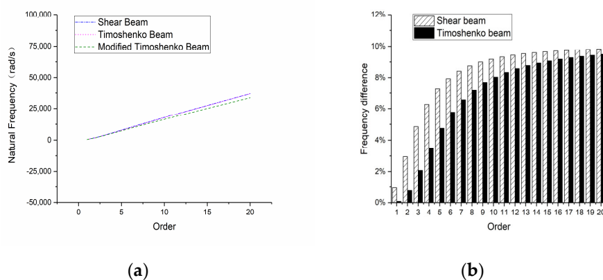
Figure 14. Natural frequencies of the 4-m-long beam: (a) overall frequency curve and (b) frequency difference compared with a modified Timoshenko beam.
