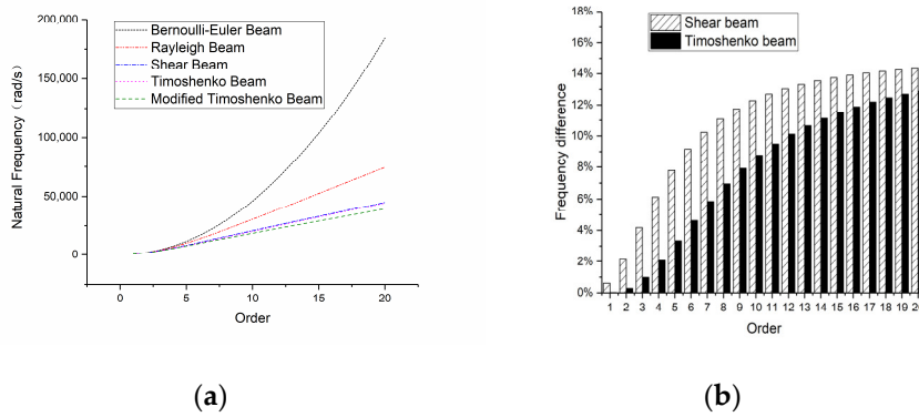
Figure 5. Natural frequencies of the 4-m-long beam: (a) overall frequency curve and (b) frequency difference compared with a modified Timoshenko beam.
