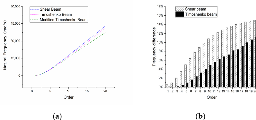
Figure 29. Natural frequencies of the 4-m-long beam: (a) overall frequency curve and (b) frequency difference compared with a modified Timoshenko beam.
