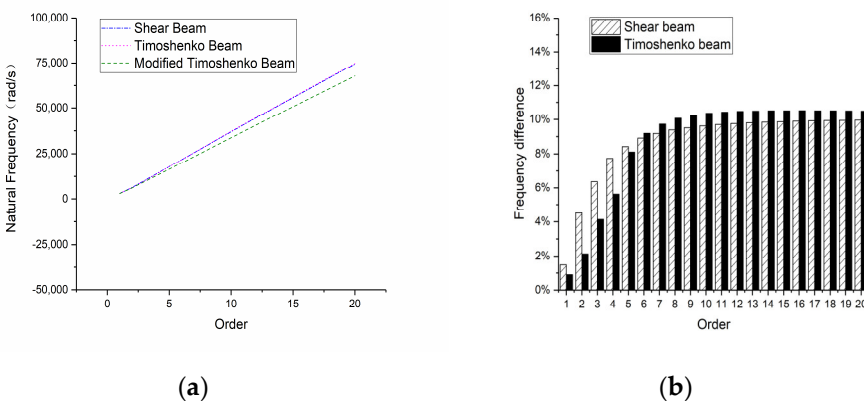
Figure 18. Natural frequencies of the 2-m-long beam: (a) overall frequency curve and (b) frequency difference compared with a modified Timoshenko beam.
