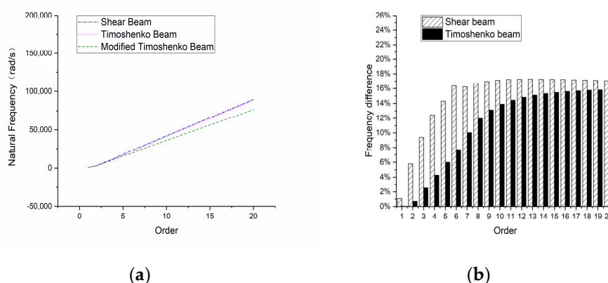
Figure 12. Natural frequencies of the 2-m-long beam: (a) overall frequency curve and (b) frequency difference compared with a modified Timoshenko beam.
