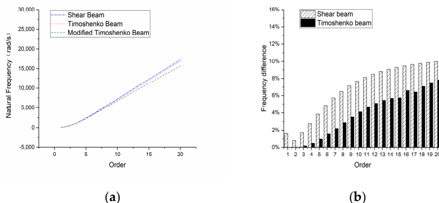
Figure 19. Natural frequencies of the 8-m-long beam: (a) overall frequency curve and (b) frequency difference compared with a modified Timoshenko beam.
