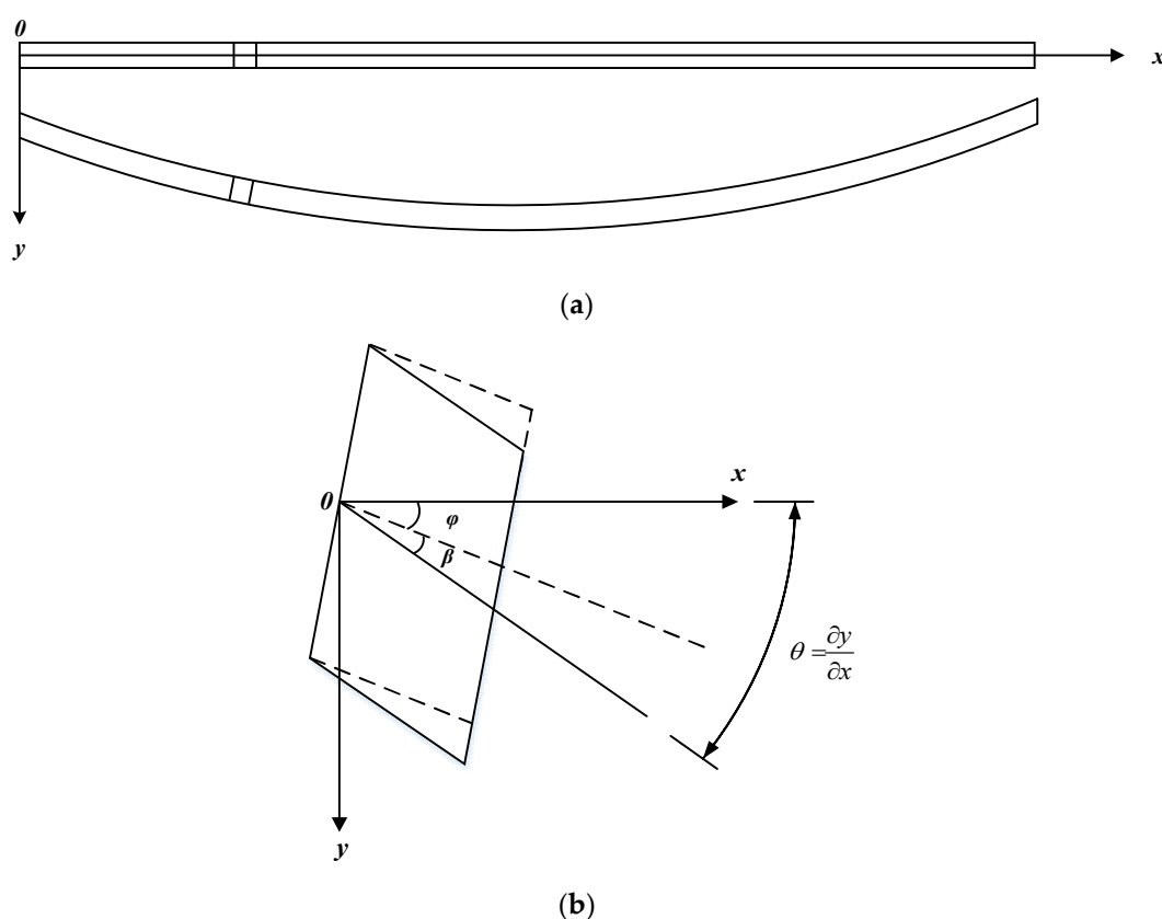
Figure 1. Deformation of the modified Timoshenko beam and a differential element diagram: (a) the lateral deformation under lateral load and (b) the element deformation.
