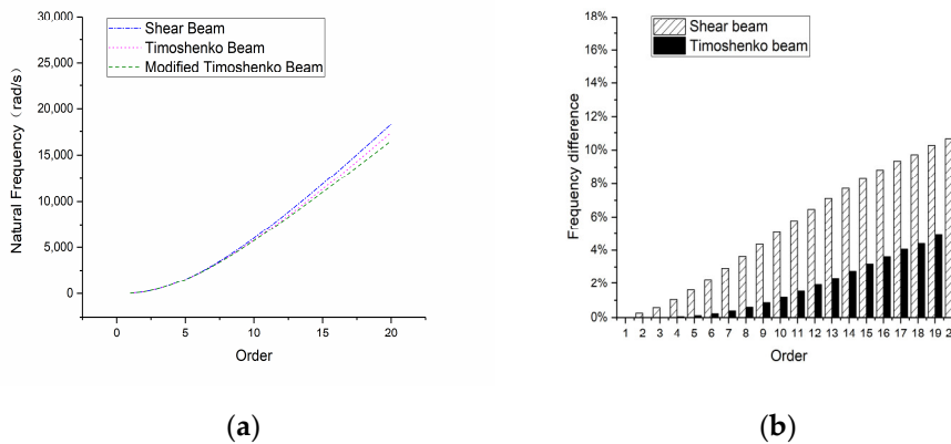
Figure 28. Natural frequencies of the 8-m-long beam: (a) overall frequency curve and (b) frequency difference compared with a modified Timoshenko beam.
