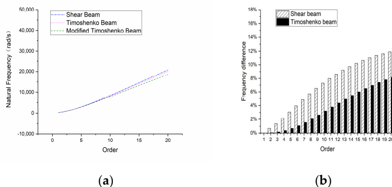
Figure 7. Natural frequencies of the 8-m-long beam: (a) overall frequency curve and (b) frequency difference compared with a modified Timoshenko beam.
