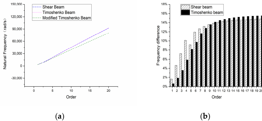
Figure 9. Natural frequencies of the 2-m-long beam: (a) overall frequency curve and (b) frequency difference compared with a modified Timoshenko beam.
