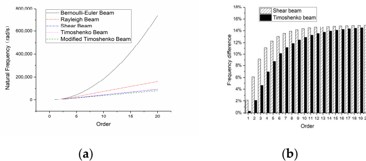
Figure 6. Natural frequencies of the 2-m-long beam: (a) overall frequency curve and (b) frequency difference compared with a modified Timoshenko beam.
