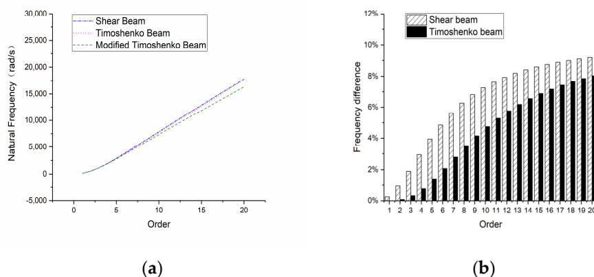
Figure 13. Natural frequencies of the 8-m-long beam: (a) overall frequency curve and (b) frequency difference compared with a modified Timoshenko beam
