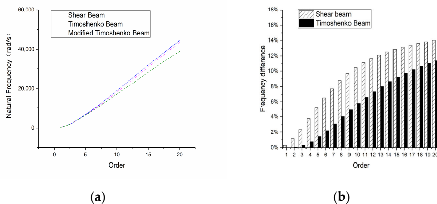
Figure 23. Natural frequencies of the 4-m-long beam: (a) overall frequency curve and (b) frequency difference compared with a modified Timoshenko beam.
