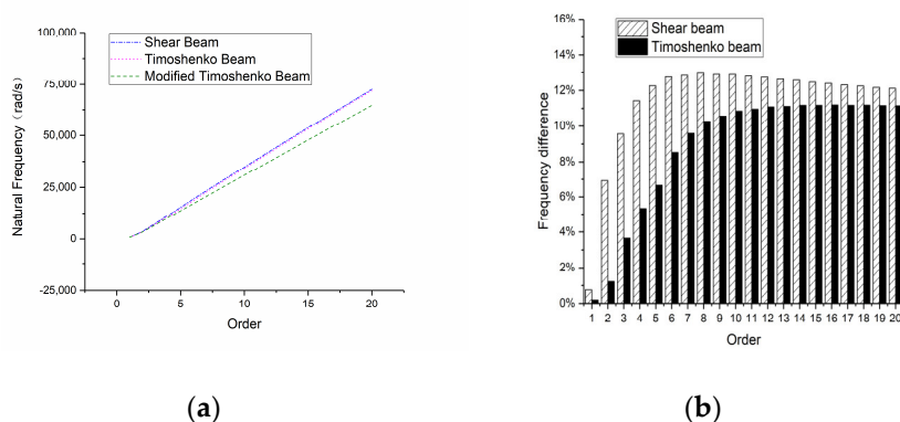
Figure 21. Natural frequencies of the 2-m-long beam: (a) overall frequency curve and (b) frequency difference compared with a modified Timoshenko beam.
