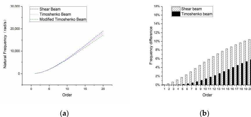
Figure 22. Natural frequencies of the 8-m-long beam: (a) overall frequency curve and (b) frequency difference compared with a modified Timoshenko beam.
