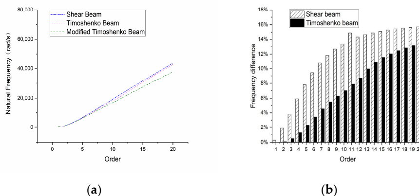
Figure 11. Natural frequencies of the 4-m-long beam: (a) overall frequency curve and (b) frequency difference compared with a modified Timoshenko beam.
