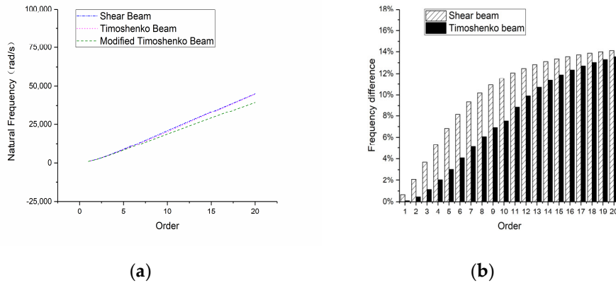
Figure 8. Natural frequencies of the 4-m-long beam: (a) overall frequency curve and (b) frequency difference compared with a modified Timoshenko beam.
