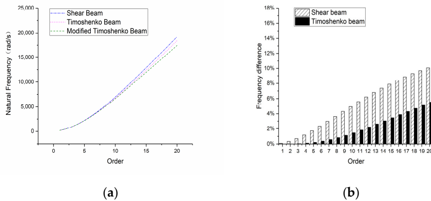
Figure 25. Natural frequencies of the 8-m-long beam: (a) overall frequency curve and (b) frequency difference compared with a modified Timoshenko beam.
