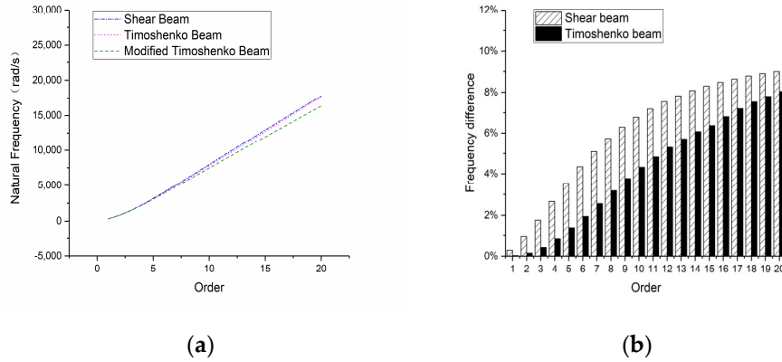
Figure 16. Natural frequencies of the 8-m-long beam: (a) overall frequency curve and (b) frequency difference compared with a modified Timoshenko beam.
