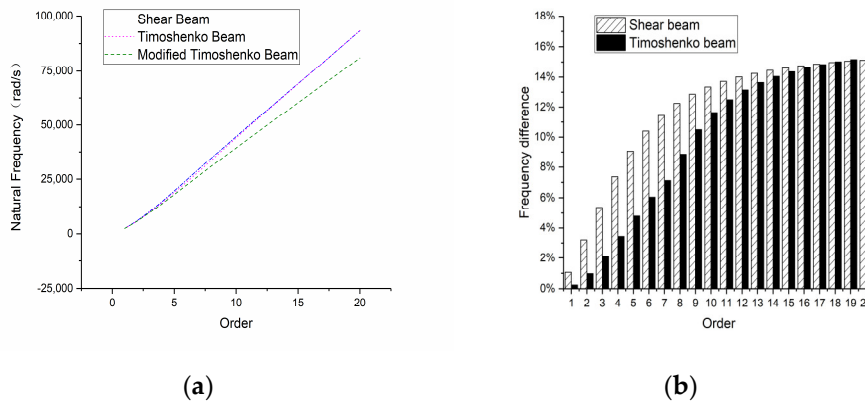
Figure 27. Natural frequencies of the 2-m-long beam: (a) overall frequency curve and (b) frequency difference compared with a modified Timoshenko beam.
