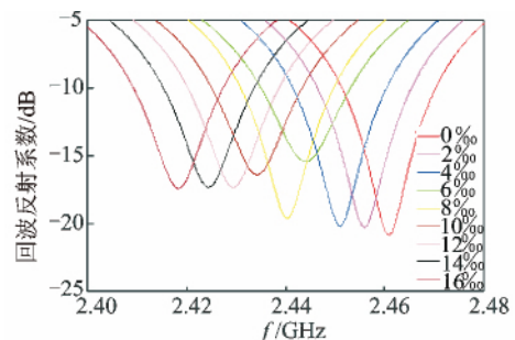
(a) 不同级别应变下模拟的 S_{11} 曲线 (a) S_{11} curves at different strain levels
