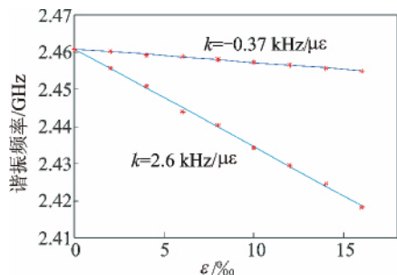
图 7 长度与宽度方向应变对天线谐振频率的影响 Fig. 7 The different impacts of length change and width change on resonance frequency shifting
