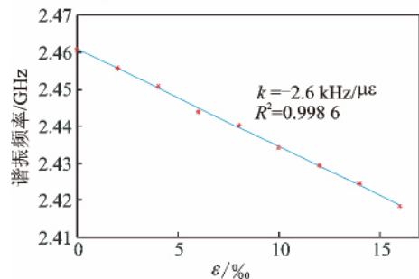
(b) 谐振频率与纵向应变之间的线性关系 (b) Linear relationship between resonance frequency and strain in length direction
