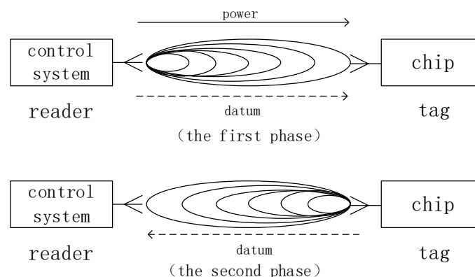
Fig.1 The operating principle of RFID system
