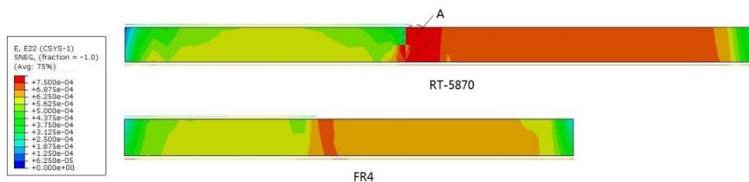
Fig. 14 Simulation result of longitudinal strain field of substrate of two antennas (lateral view in A-A' section)
