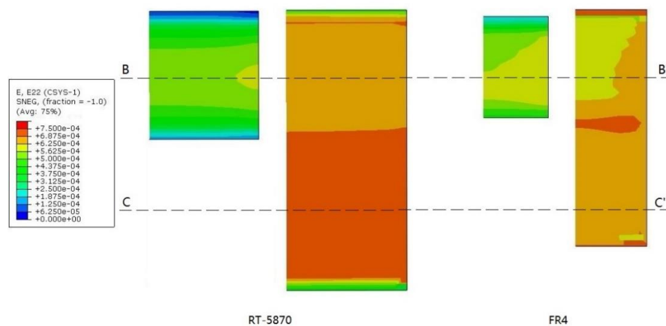
Fig. 13 Simulation result of longitudinal strain field of copper patched and ground plane of two antennas (vertical view)
