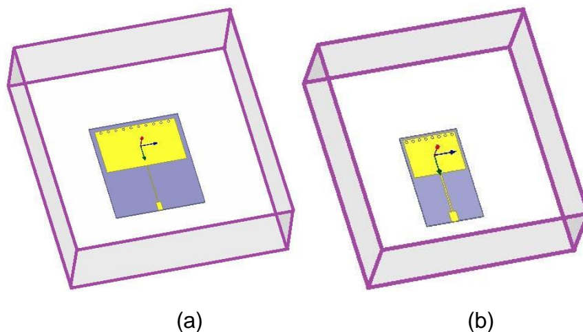
Fig. 5 3D prototypes of two patched antennas in HFSS TM . (a) RT-5870 substrate. (b) FR4 substrate
