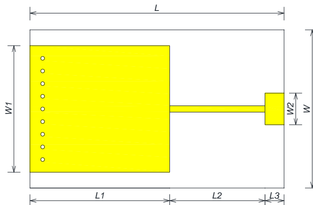
Fig. 6 Illustration of detail dimension of patched antennas
